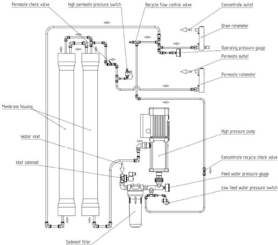
Figure 4.4 Layout of Ecosoft MO 10000
