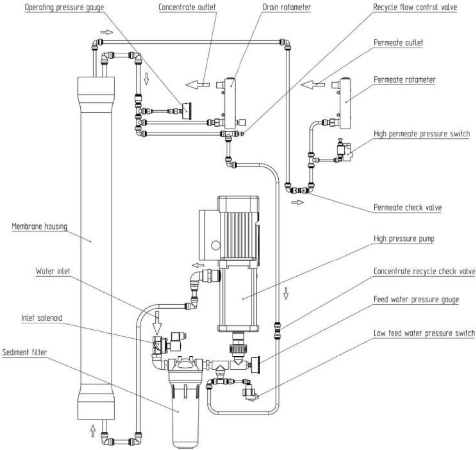
Figure 4.3 Layout of Ecosoft MO 5000
