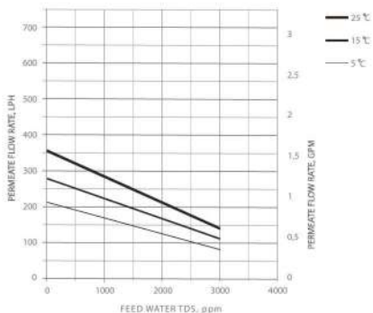
Figure 4.1 Ecosoft MO5000 flow rate chart
