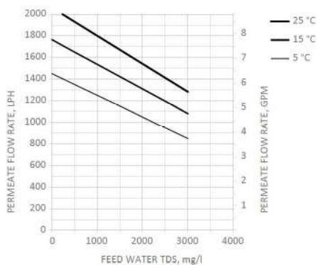
Figure 2.4 Ecosoft MO36000 flow rate chart
