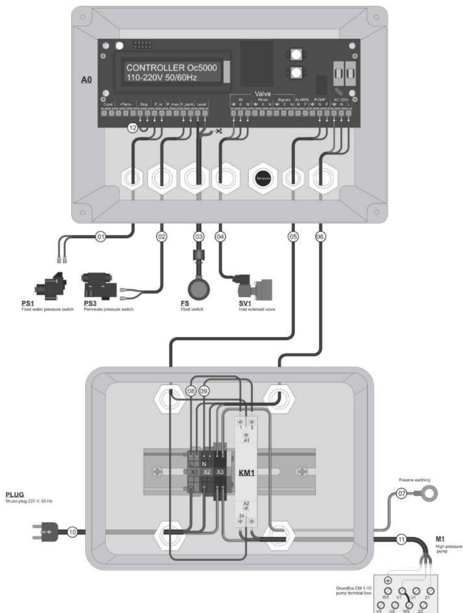
Figure 4.6 Wiring diagram
